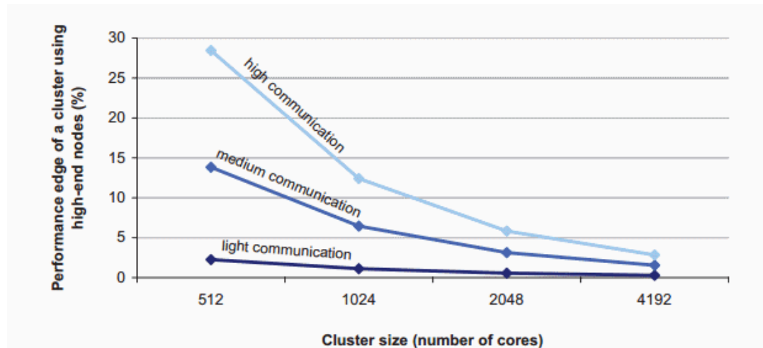
FIGURE 3.2: Performance advantage of a cluster built with high-end server nodes (128-core SMP) over a cluster with the same number of processor cores built with low-end server nodes (four-core SMP), for clusters of varying size.
